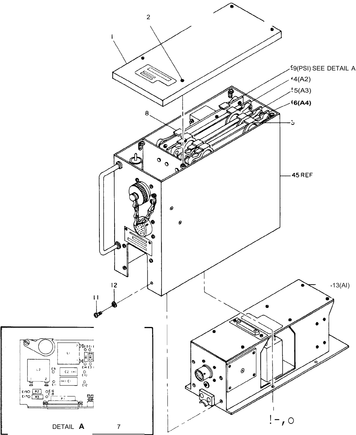
Figure 7-1. Control Unit - Exploded View (Sheet 1 of 2)
