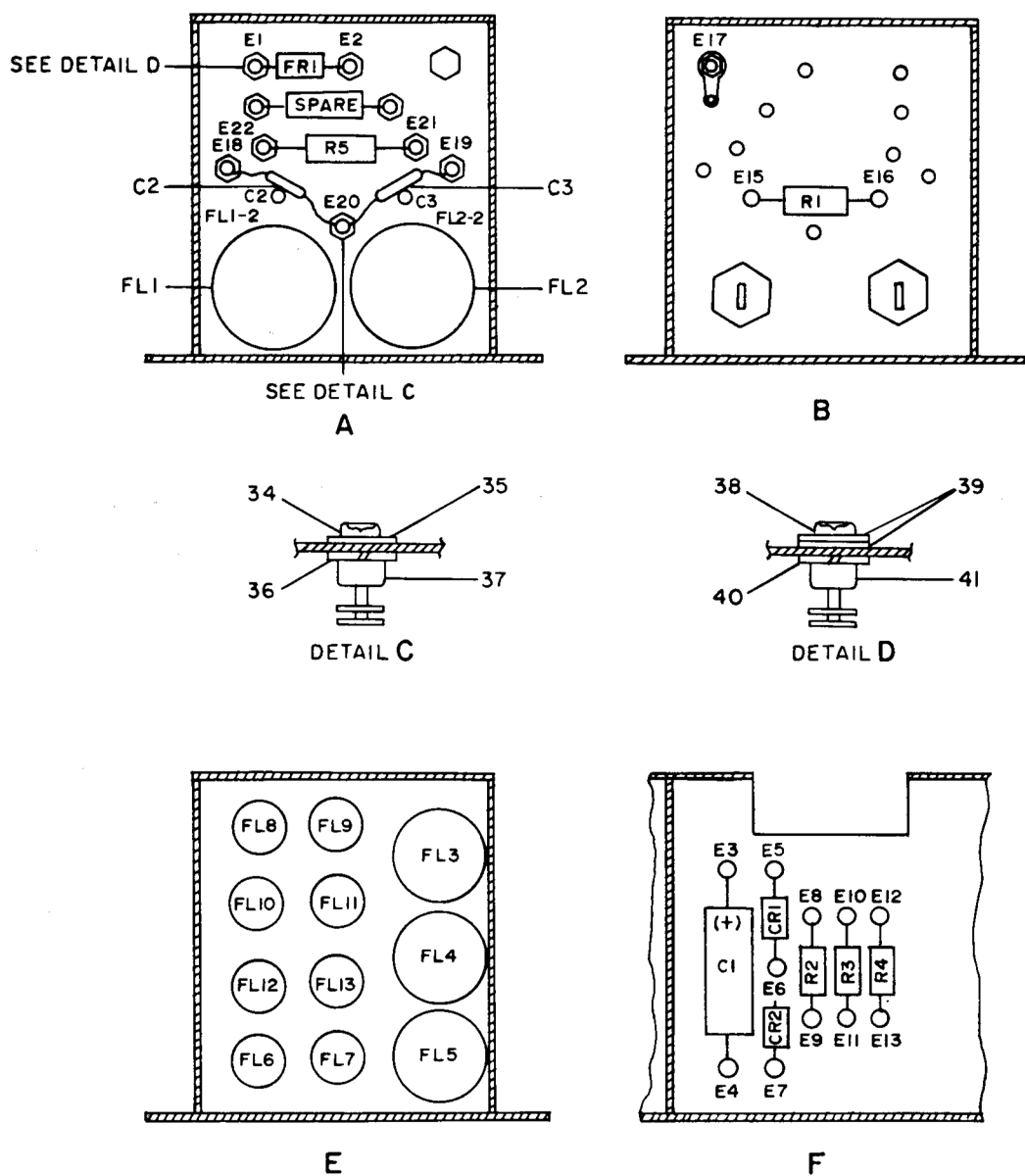
Figure 8-1. Component Module Assembly (A1) (Sheet 2)
