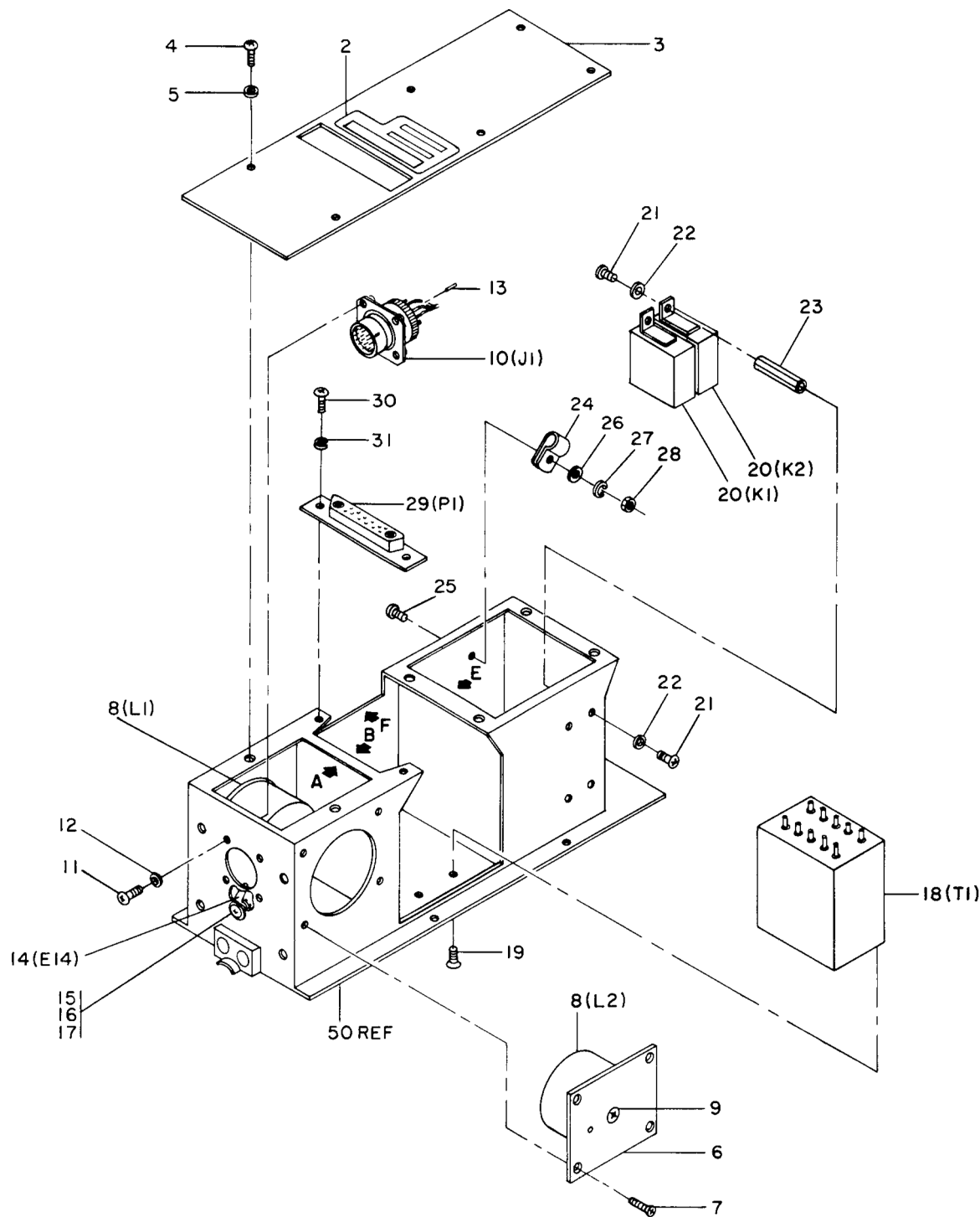
Figure 9-2. Module Assembly (A1), Component (Sheet 1 of 2)
