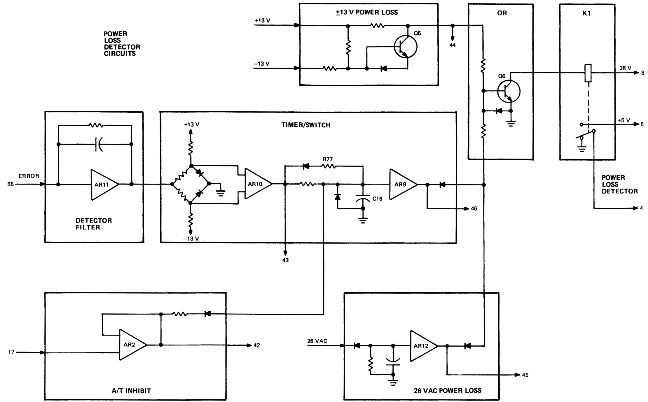
FO-2. CCA A2 - Simplified Block Diagram (Sheet 2)
