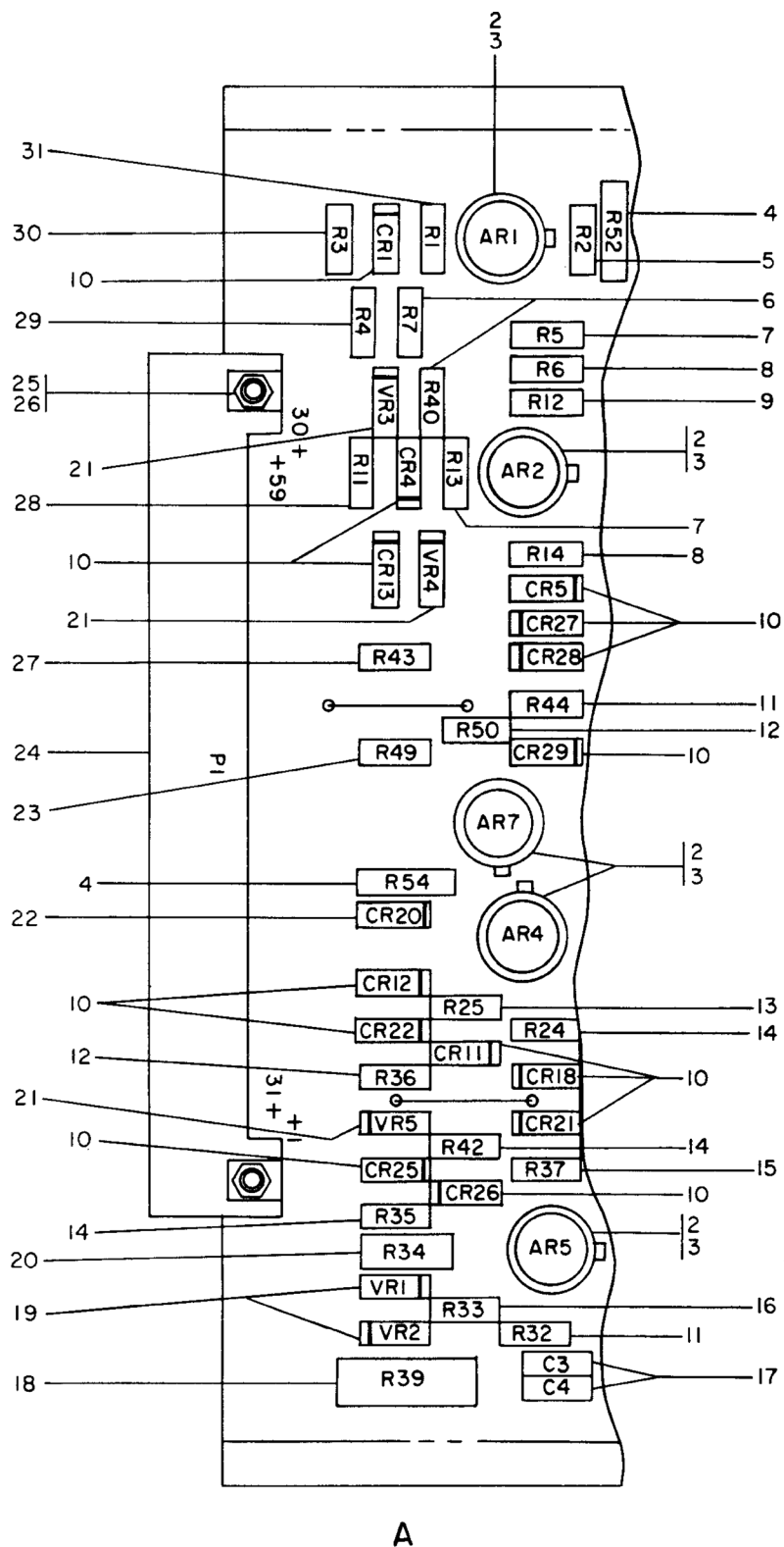
Figure 9-4. Circuit Card Assembly (A3) (Sheet 1 of 2)
