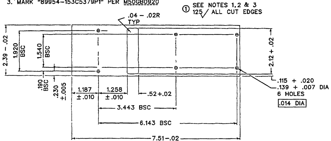
Figure 8-4. Module Cover
