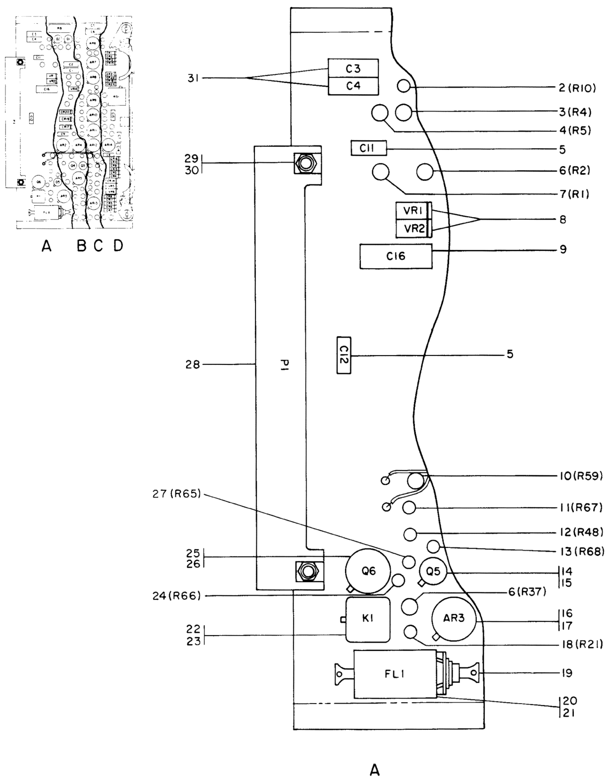
Figure 9-3. Circuit Card Assembly (A2) (Sheet 1 of 3)
